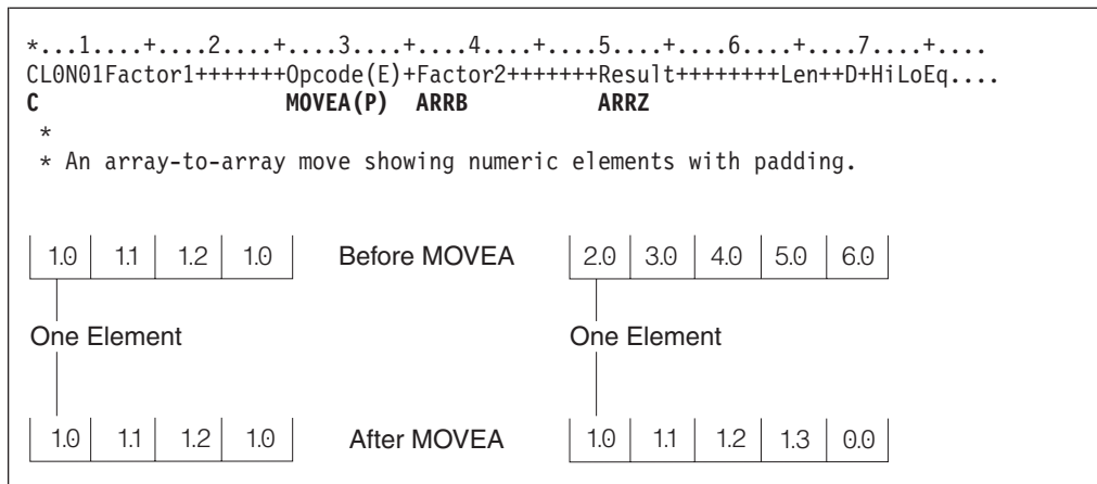
Figure 346. MOVEA Operation (Part 9 of 10)
