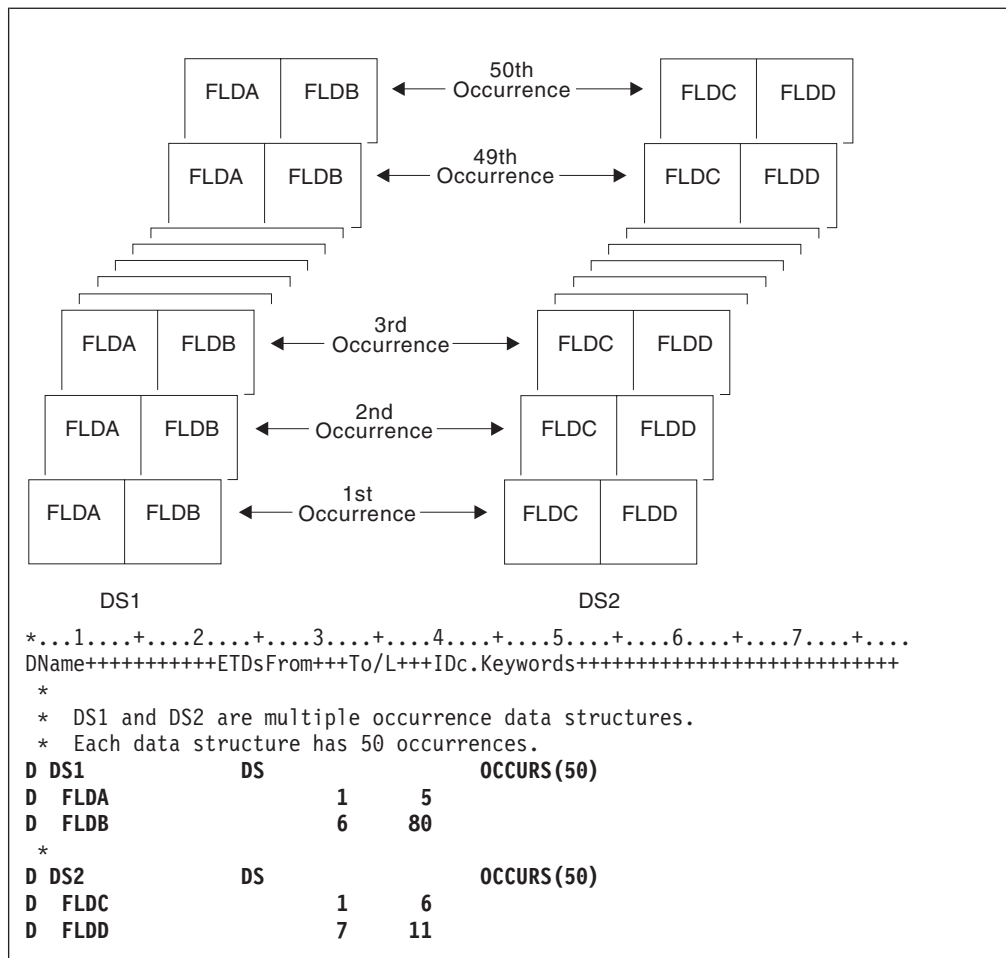
Figure 357. Uses of the OCCUR Operation (Part 1 of 2)
