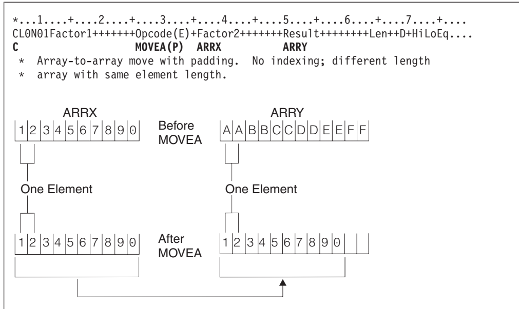
Figure 346. MOVEA Operation (Part 8 of 10)
