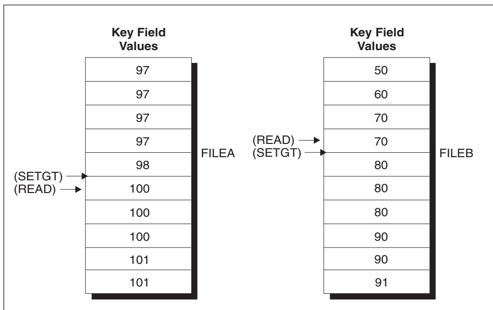
Figure 377. SETGT Operation (Part 2 of 4)
