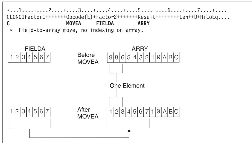
Figure 346. MOVEA Operation (Part 5 of 10)
