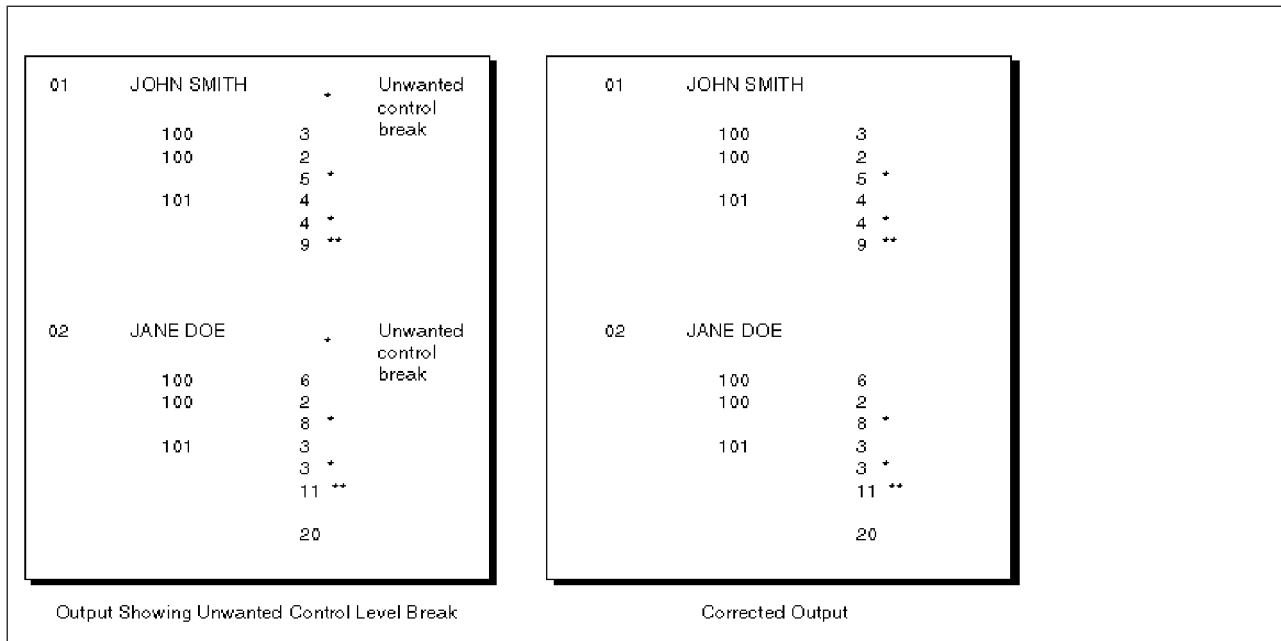
Figure 17. How to Avoid Unwanted Control Breaks (Part 4 of 4)
