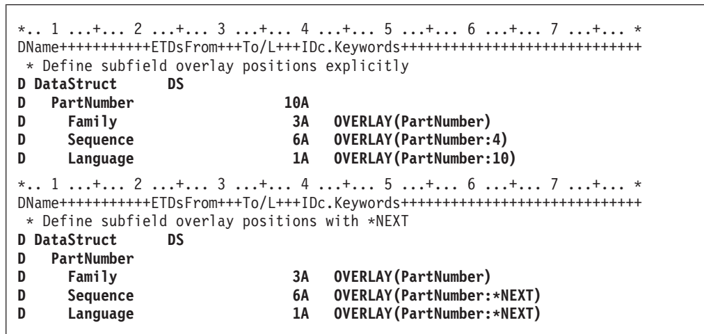
Figure 146. Defining Subfield Overlay Positions with *NEXT
